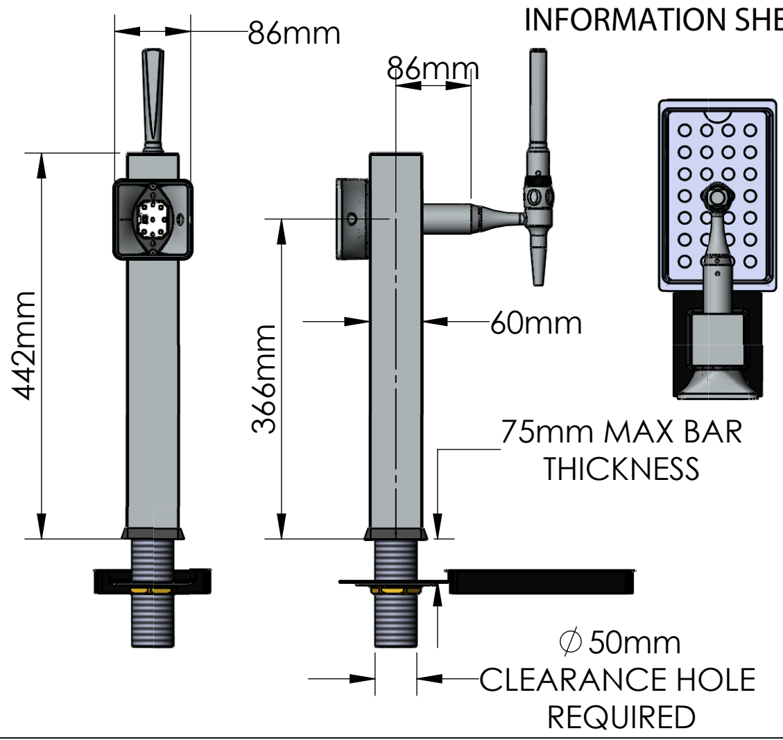
STANDARD HEIGHT THROUGH BAR
