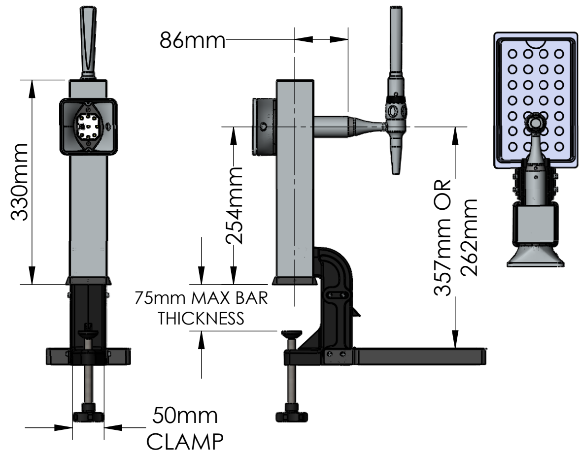
LOWPLAZA CLAMP-ON
