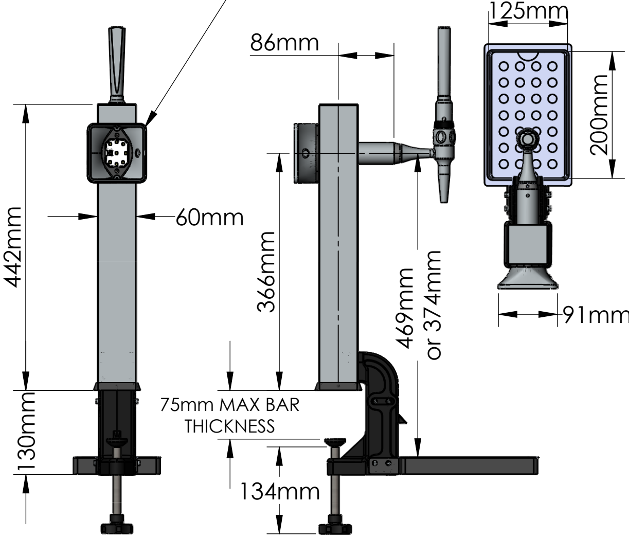
STANDARD HEIGHT CLAMP-ON
