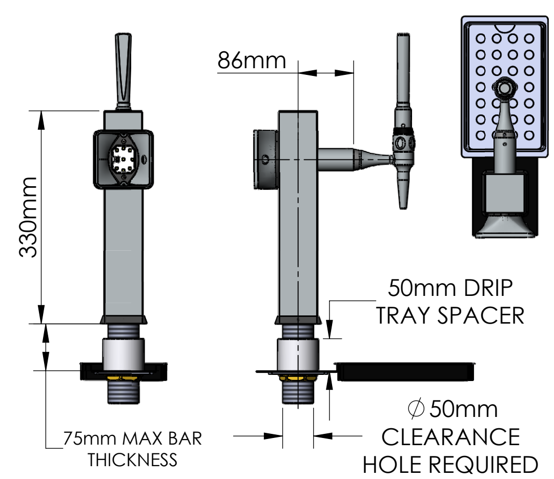
LOWPLAZA THROUGH BAR
